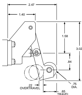
Lever-Roller-KR2
