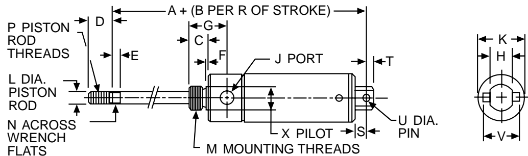
ALL DIMENSIONS IN INCHES
