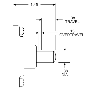
Tappet-KP0
