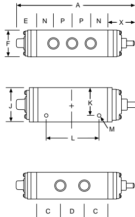
DIMENSIONS — VALVE WITH MANUAL OPERATOR — ALL DIMENSIONS IN INCHES
